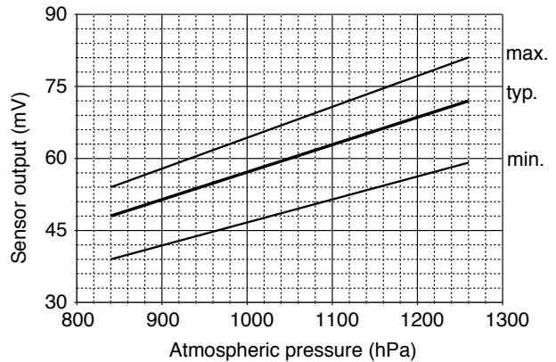
Fig. 5 - KE-50 response of output voltage to ambient pressure changes (at 25°C/60%RH)
