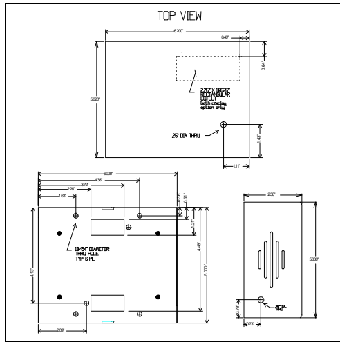
Figure 1 Optional Enclosure Dimensions
